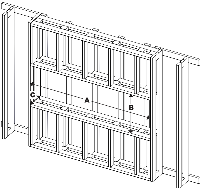
VST130-I Installation
