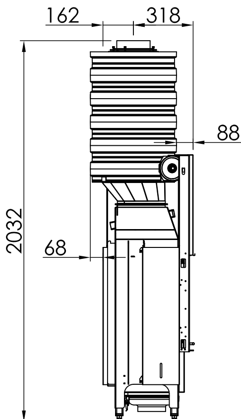
~1:20 Rear outlet, Eccentric adapter
